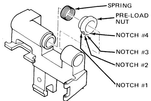
FIGURE 8 CARRIAGE ASSEMBLY
