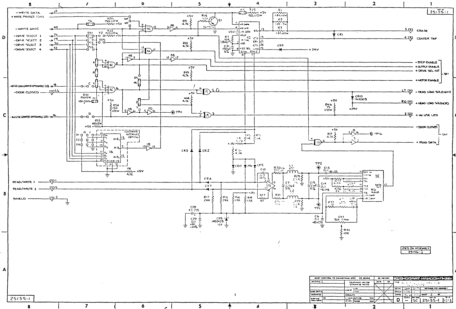
FIGURE 6-3. SCHEMATIC DIAGRAM, P/N 25136 (SHEET 2 OF 2)
