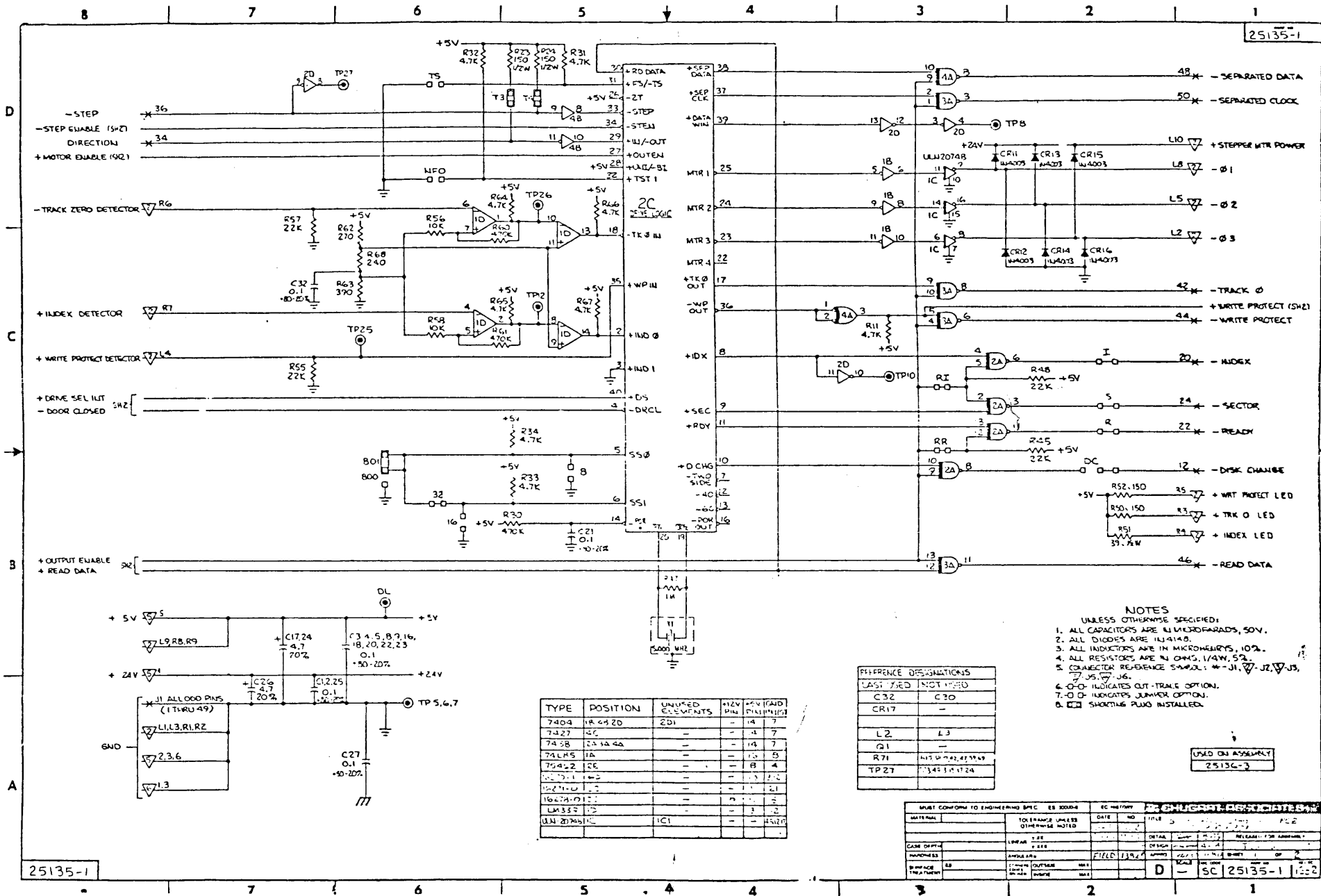
FIGURE 6-3. SCHEMATIC DIAGRAM, P/N 25136 (SHEET 1 OF 2)
